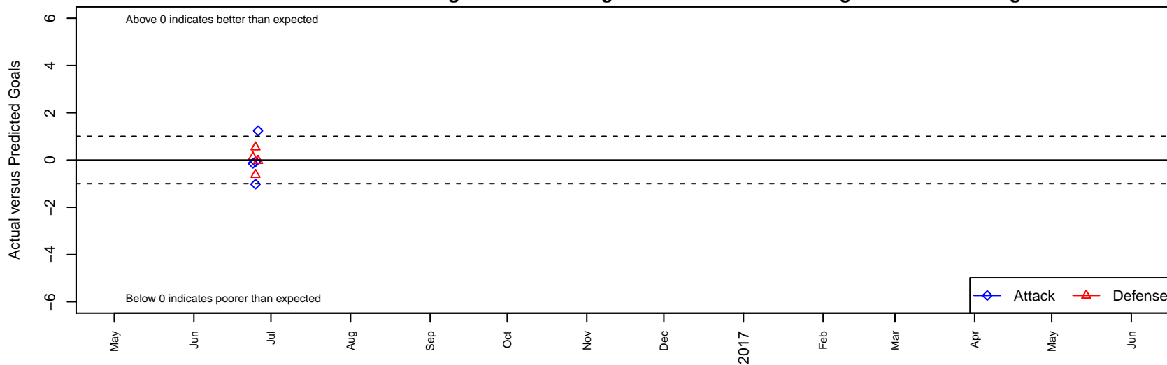
Ridgeview HS Ravens B98 Dots are actual minus expected GF (blue circles) and GA (red triangles). Blue line is smoothed change in attack strength. Red is smoothed change in defense strength.
